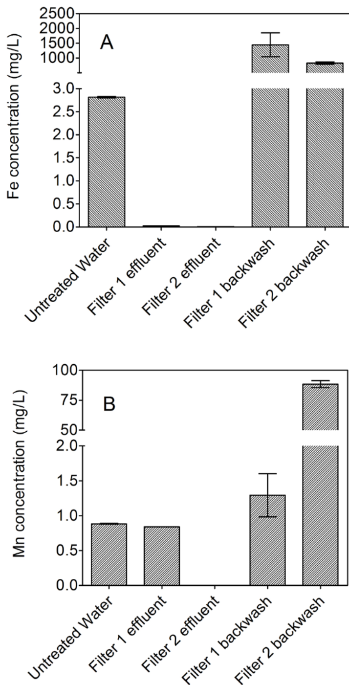
Figure 1: Iron and manganese concentrations of different water samples from the filtration unit: A. The change in the iron concentration in the effluents of the filtration unit, B. The change in the manganese concentration in the effluents of the filtration unit.
