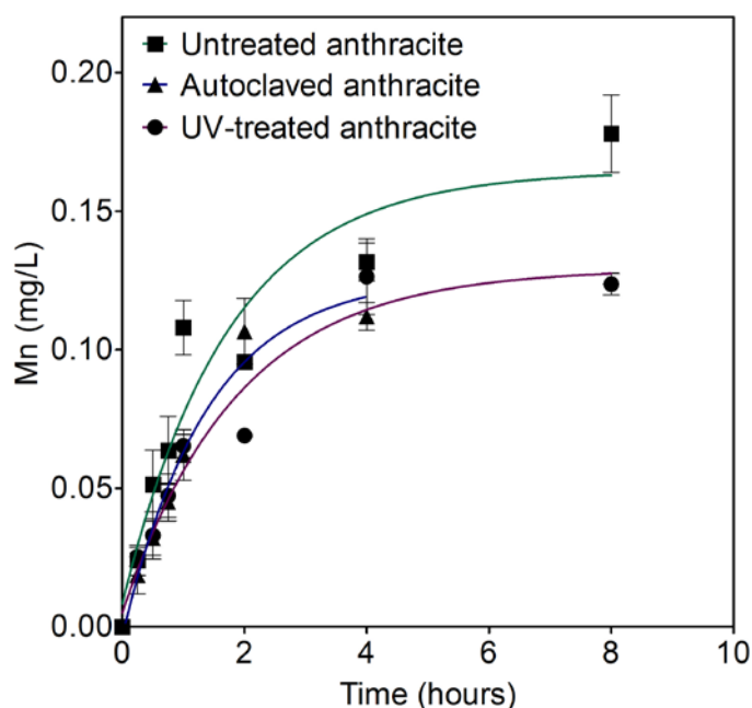
Figure 4: Mn (II) concentrations in solid phase (adsorbed to anthracite) over time for UV-treated, autoclaved and untreated anthracite at 22 °C.
